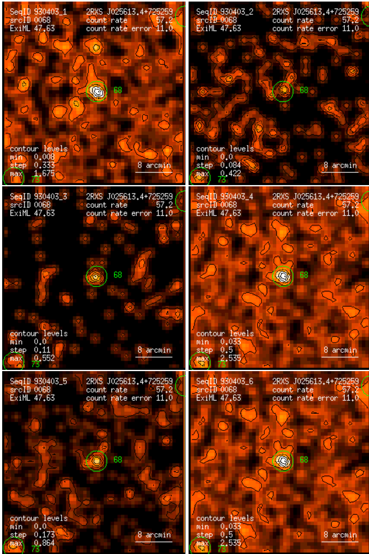
Figure 68: RASS 930403: detection 0068: band rate images, Gaussian filter: (1) PSPC channels 11 – 41, (2) 52 – 90, (3) 91 – 201, (4) 11 – 235, (5) 52 – 201, (6) 11 – 201. Broad band rates in counts/ks. Band rate contour levels in counts/ks/arcmin 2 .
