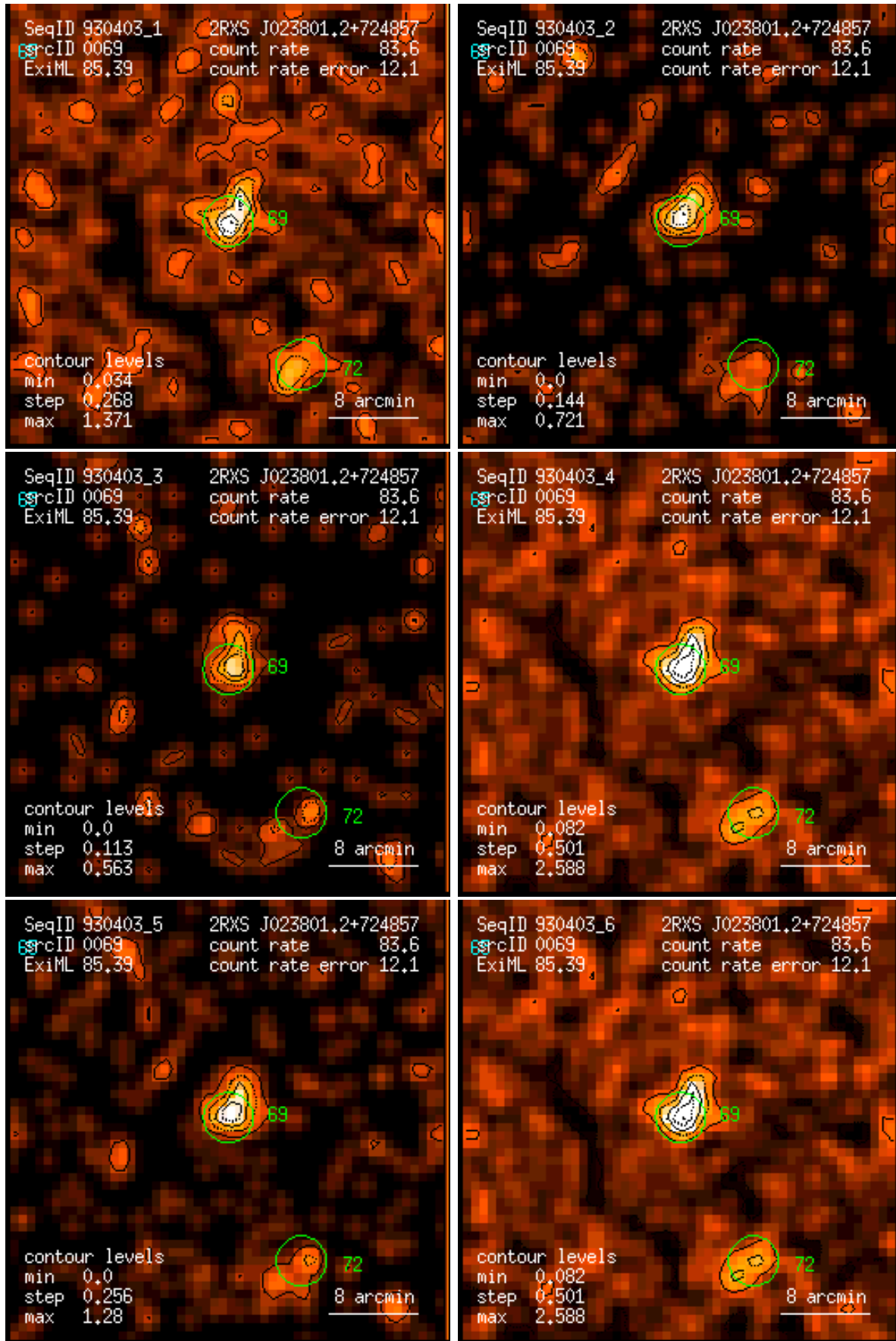
Figure 69: RASS 930403: detection 0069: band rate images, Gaussian filter: (1) PSPC channels 11 – 41, (2) 52 – 90, (3) 91 – 201, (4) 11 – 235, (5) 52 – 201, (6) 11 – 201. Broad band rates in counts/ks. Band rate contour levels in counts/ks/arcmin 2 .
