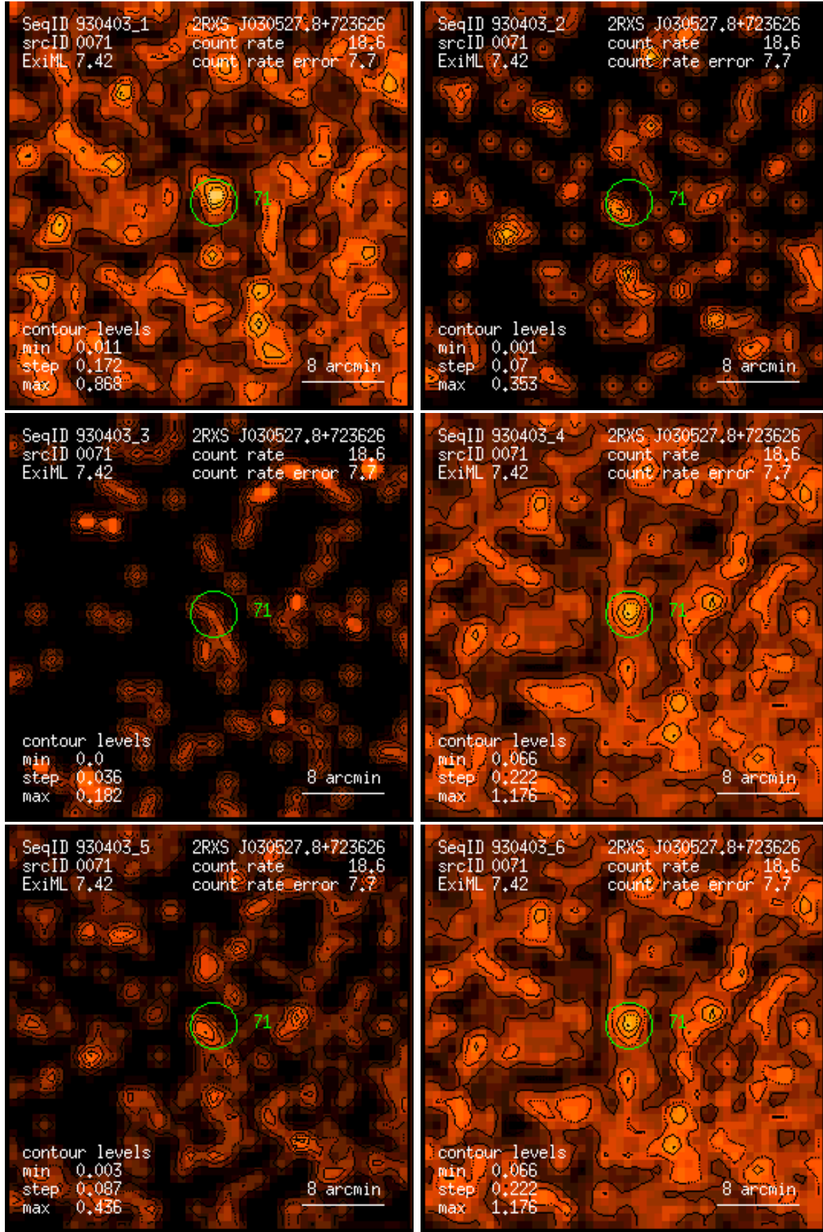
Figure 71: RASS 930403: detection 0071: band rate images, Gaussian filter: (1) PSPC channels 11 – 41, (2) 52 – 90, (3) 91 – 201, (4) 11 – 235, (5) 52 – 201, (6) 11 – 201. Broad band rates in counts/ks. Band rate contour levels in counts/ks/arcmin 2 .
