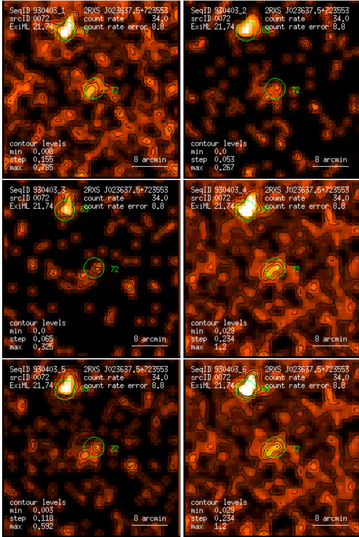
Figure 72: RASS 930403: detection 0072: band rate images, Gaussian filter: (1) PSPC channels 11 – 41, (2) 52 – 90, (3) 91 – 201, (4) 11 – 235, (5) 52 – 201, (6) 11 – 201. Broad band rates in counts/ks. Band rate contour levels in counts/ks/arcmin 2 .
