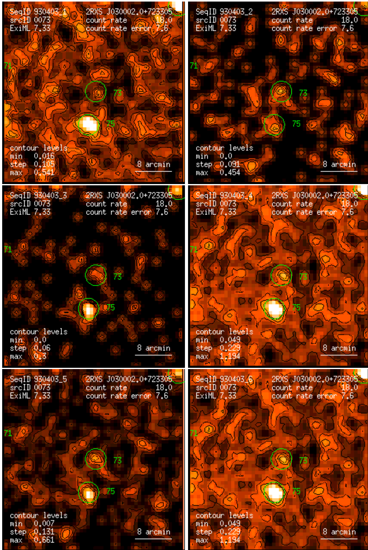
Figure 73: RASS 930403: detection 0073: band rate images, Gaussian filter: (1) PSPC channels 11 – 41, (2) 52 – 90, (3) 91 – 201, (4) 11 – 235, (5) 52 – 201, (6) 11 – 201. Broad band rates in counts/ks. Band rate contour levels in counts/ks/arcmin 2 .
