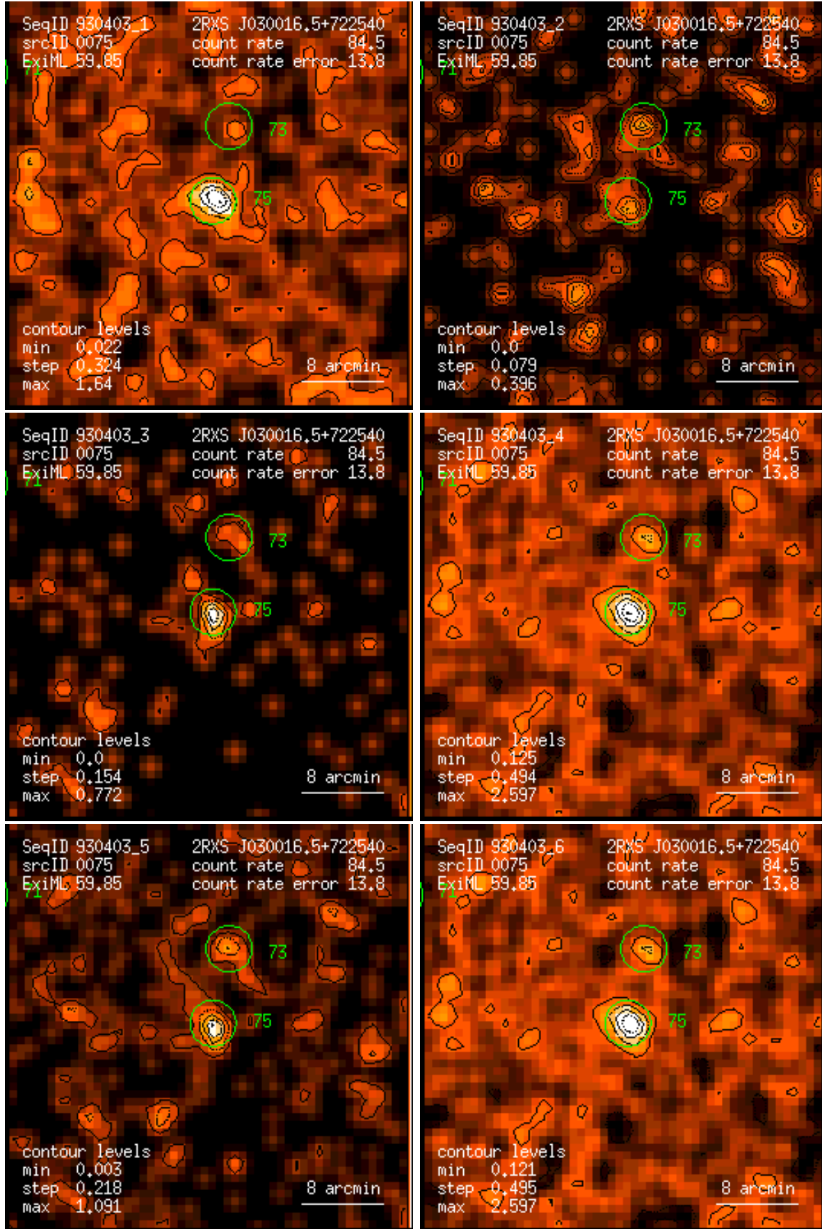
Figure 75: RASS 930403: detection 0075: band rate images, Gaussian filter: (1) PSPC channels 11 – 41, (2) 52 – 90, (3) 91 – 201, (4) 11 – 235, (5) 52 – 201, (6) 11 – 201. Broad band rates in counts/ks. Band rate contour levels in counts/ks/arcmin 2 .
