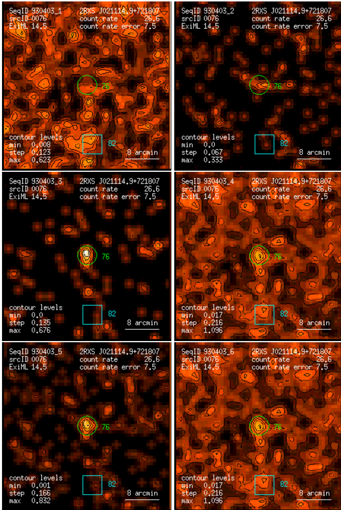
Figure 76: RASS 930403: detection 0076: band rate images, Gaussian filter: (1) PSPC channels 11 – 41, (2) 52 – 90, (3) 91 – 201, (4) 11 – 235, (5) 52 – 201, (6) 11 – 201. Broad band rates in counts/ks. Band rate contour levels in counts/ks/arcmin 2 .
