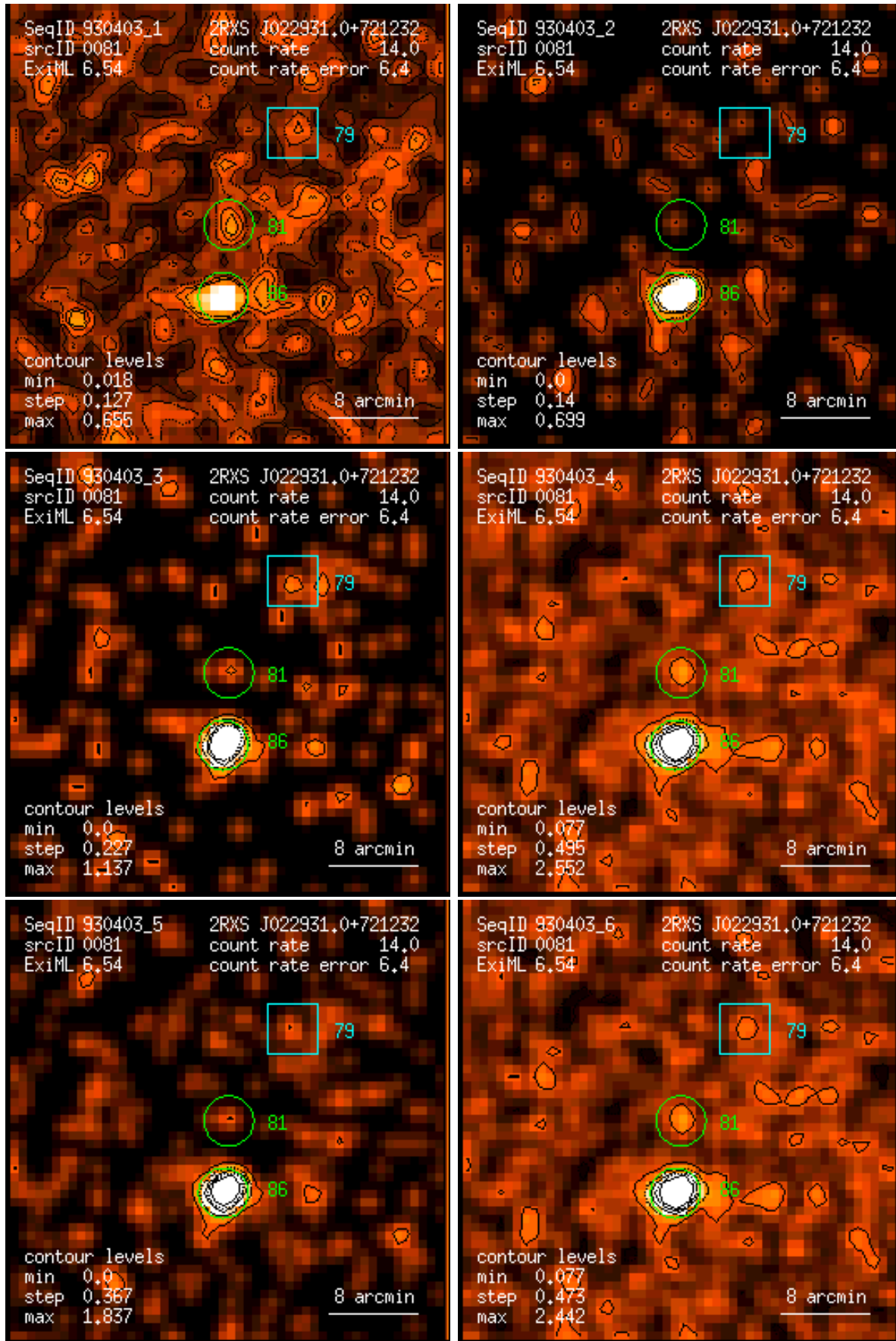
Figure 81: RASS 930403: detection 0081: band rate images, Gaussian filter: (1) PSPC channels 11 – 41, (2) 52 – 90, (3) 91 – 201, (4) 11 – 235, (5) 52 – 201, (6) 11 – 201. Broad band rates in counts/ks. Band rate contour levels in counts/ks/arcmin 2 .
