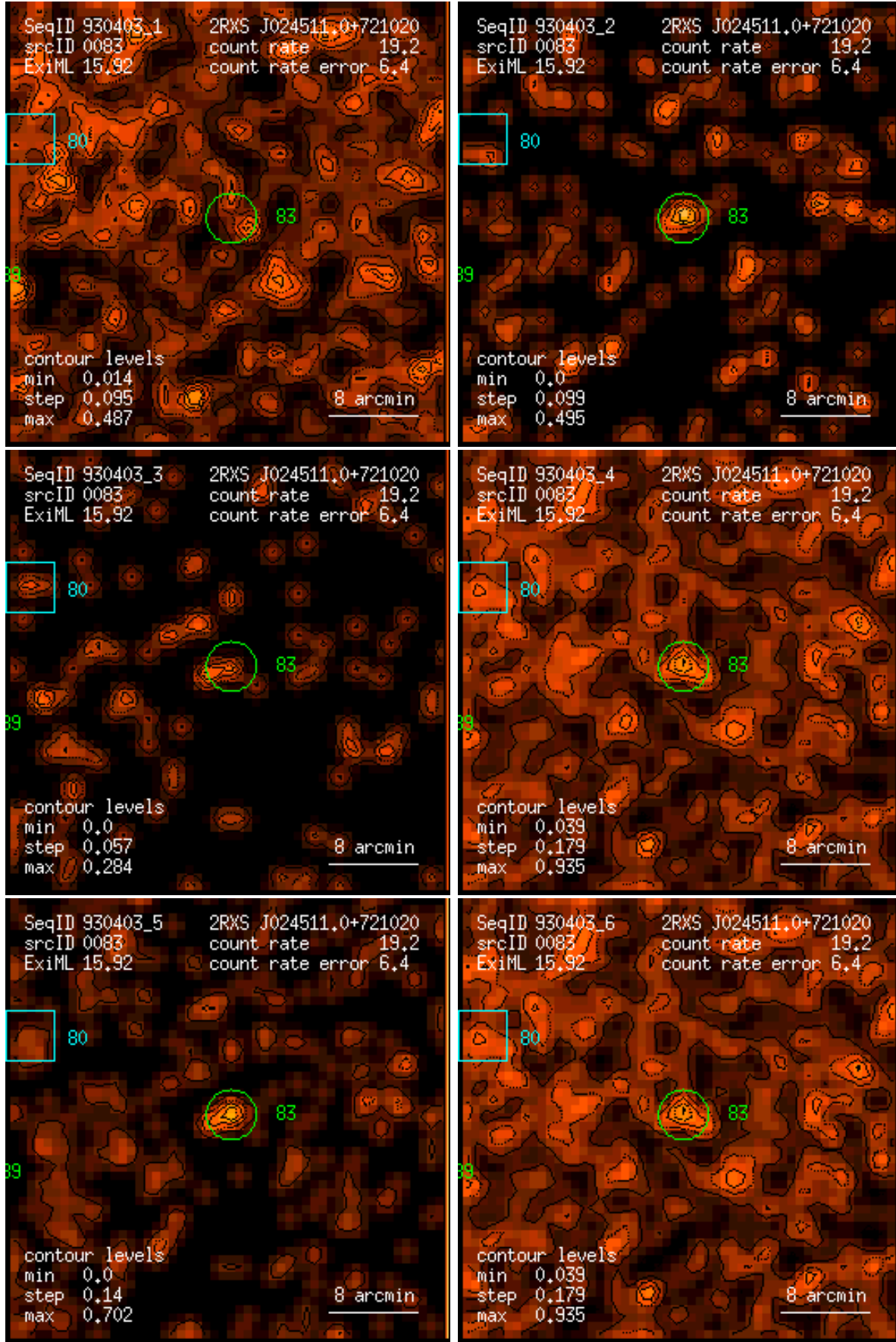
Figure 83: RASS 930403: detection 0083: band rate images, Gaussian filter: (1) PSPC channels 11 – 41, (2) 52 – 90, (3) 91 – 201, (4) 11 – 235, (5) 52 – 201, (6) 11 – 201. Broad band rates in counts/ks. Band rate contour levels in counts/ks/arcmin 2 .
