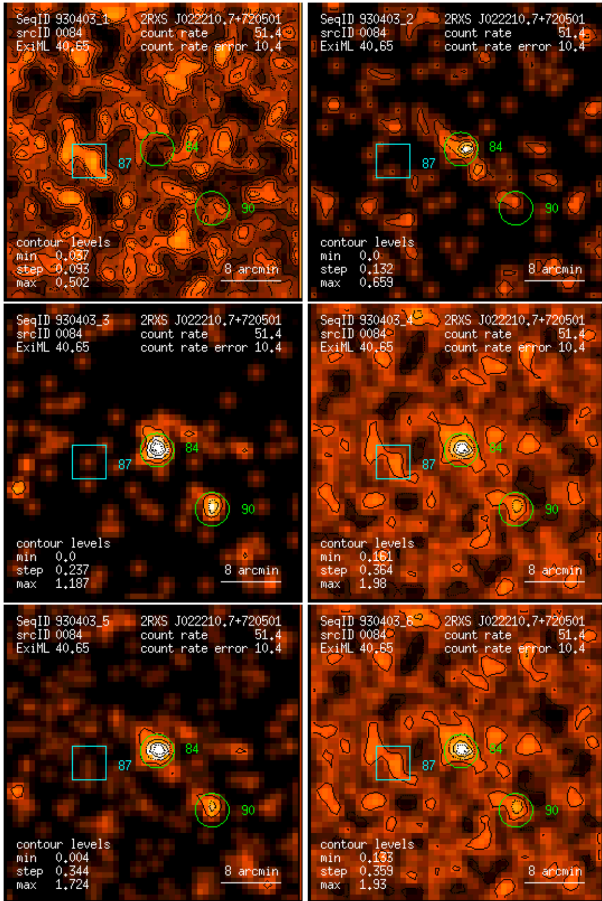
Figure 84: RASS 930403: detection 0084: band rate images, Gaussian filter: (1) PSPC channels 11 – 41, (2) 52 – 90, (3) 91 – 201, (4) 11 – 235, (5) 52 – 201, (6) 11 – 201. Broad band rates in counts/ks. Band rate contour levels in counts/ks/arcmin 2 .
