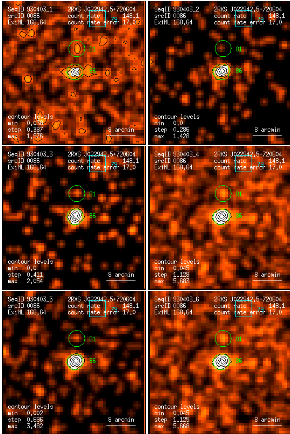
Figure 86: RASS 930403: detection 0086: band rate images, Gaussian filter: (1) PSPC channels 11 – 41, (2) 52 – 90, (3) 91 – 201, (4) 11 – 235, (5) 52 – 201, (6) 11 – 201. Broad band rates in counts/ks. Band rate contour levels in counts/ks/arcmin 2 .
