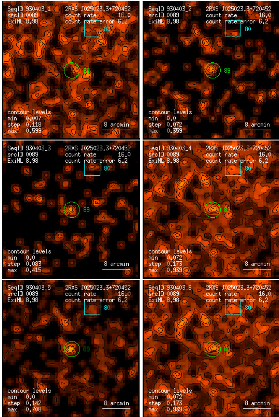
Figure 89: RASS 930403: detection 0089: band rate images, Gaussian filter: (1) PSPC channels 11 – 41, (2) 52 – 90, (3) 91 – 201, (4) 11 – 235, (5) 52 – 201, (6) 11 – 201. Broad band rates in counts/ks. Band rate contour levels in counts/ks/arcmin 2 .
