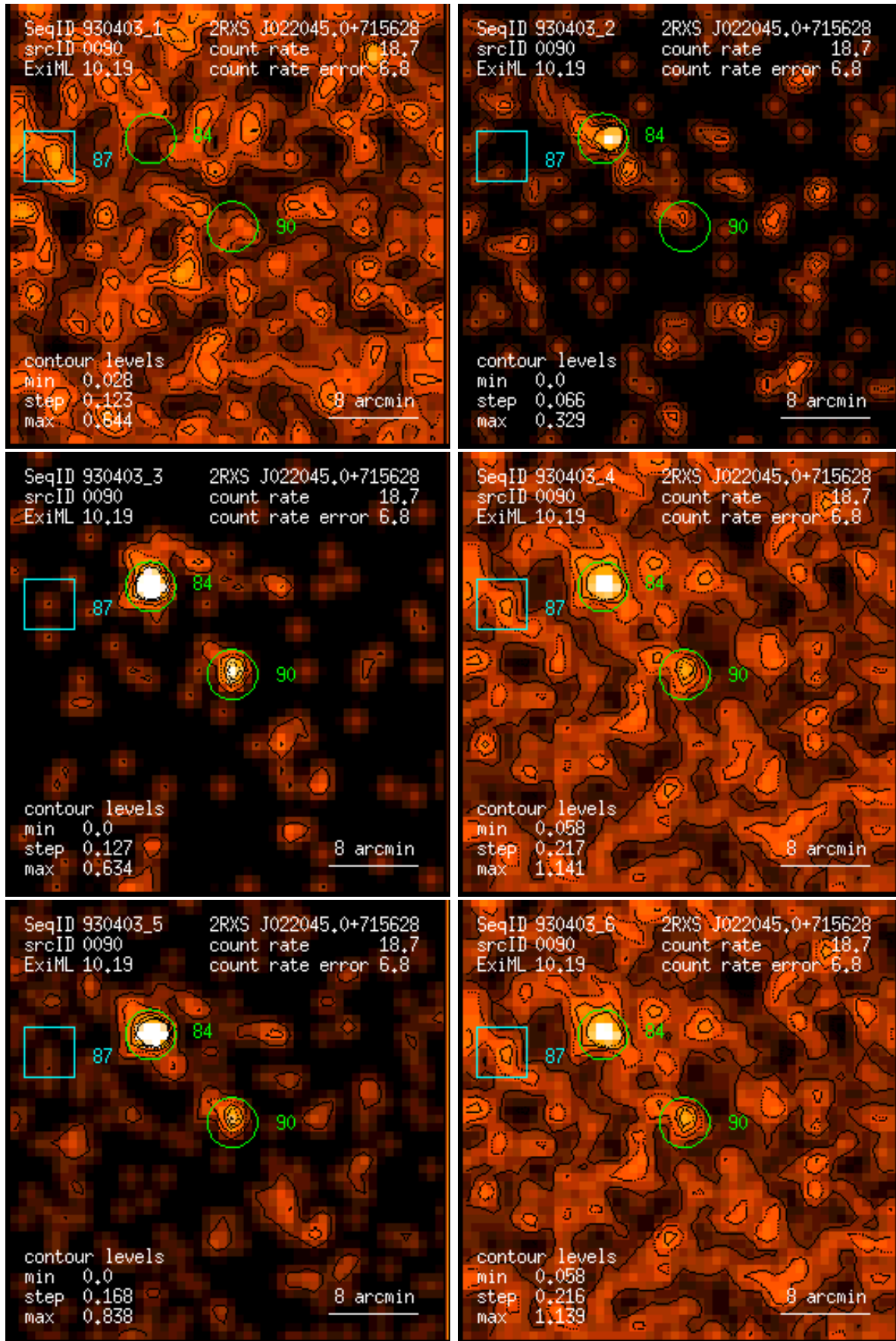
Figure 90: RASS 930403: detection 0090: band rate images, Gaussian filter: (1) PSPC channels 11 – 41, (2) 52 – 90, (3) 91 – 201, (4) 11 – 235, (5) 52 – 201, (6) 11 – 201. Broad band rates in counts/ks. Band rate contour levels in counts/ks/arcmin 2 .
