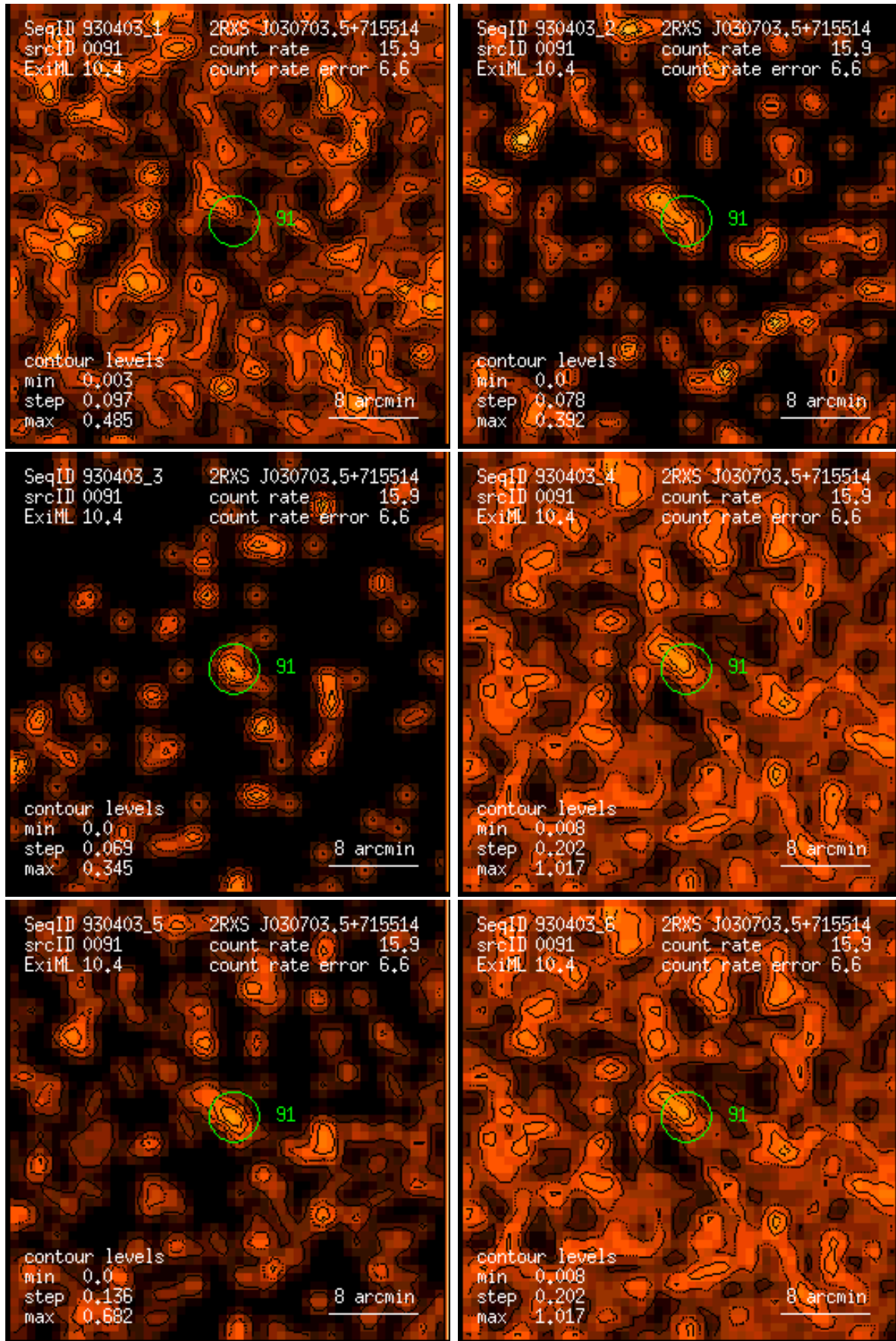
Figure 91: RASS 930403: detection 0091: band rate images, Gaussian filter: (1) PSPC channels 11 – 41, (2) 52 – 90, (3) 91 – 201, (4) 11 – 235, (5) 52 – 201, (6) 11 – 201. Broad band rates in counts/ks. Band rate contour levels in counts/ks/arcmin 2 .
