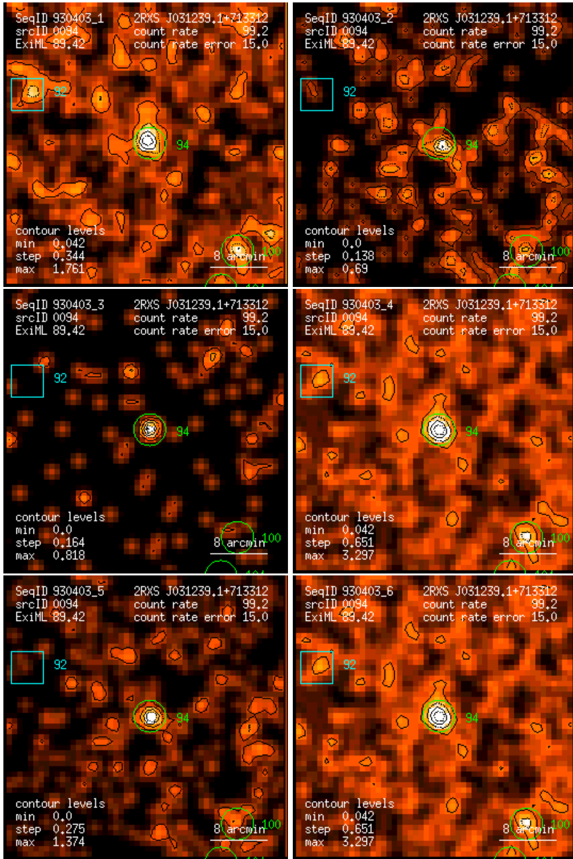
Figure 94: RASS 930403: detection 0094: band rate images, Gaussian filter: (1) PSPC channels 11 – 41, (2) 52 – 90, (3) 91 – 201, (4) 11 – 235, (5) 52 – 201, (6) 11 – 201. Broad band rates in counts/ks. Band rate contour levels in counts/ks/arcmin 2 .
