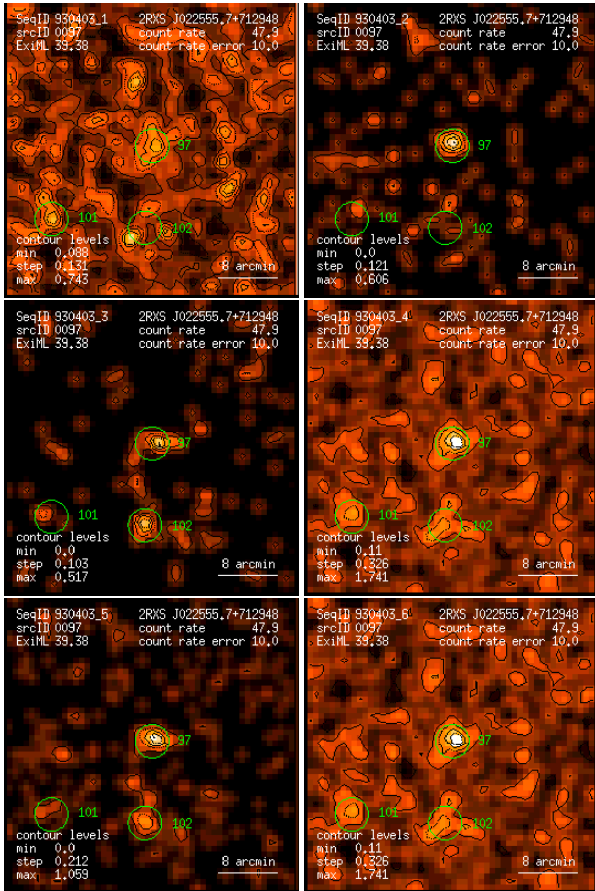
Figure 97: RASS 930403: detection 0097: band rate images, Gaussian filter: (1) PSPC channels 11 – 41, (2) 52 – 90, (3) 91 – 201, (4) 11 – 235, (5) 52 – 201, (6) 11 – 201. Broad band rates in counts/ks. Band rate contour levels in counts/ks/arcmin 2 .
