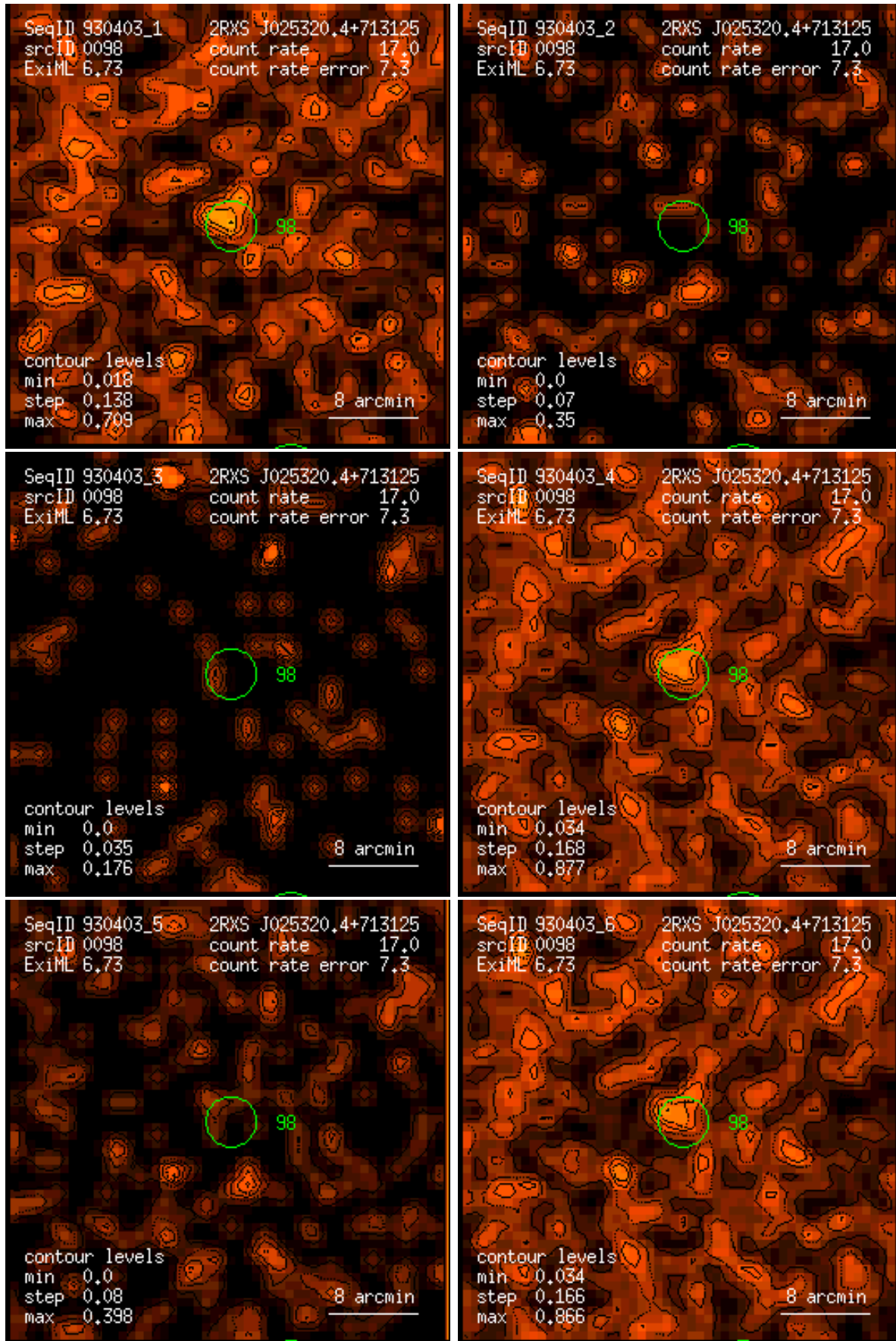
Figure 98: RASS 930403: detection 0098: band rate images, Gaussian filter: (1) PSPC channels 11 – 41, (2) 52 – 90, (3) 91 – 201, (4) 11 – 235, (5) 52 – 201, (6) 11 – 201. Broad band rates in counts/ks. Band rate contour levels in counts/ks/arcmin 2 .
