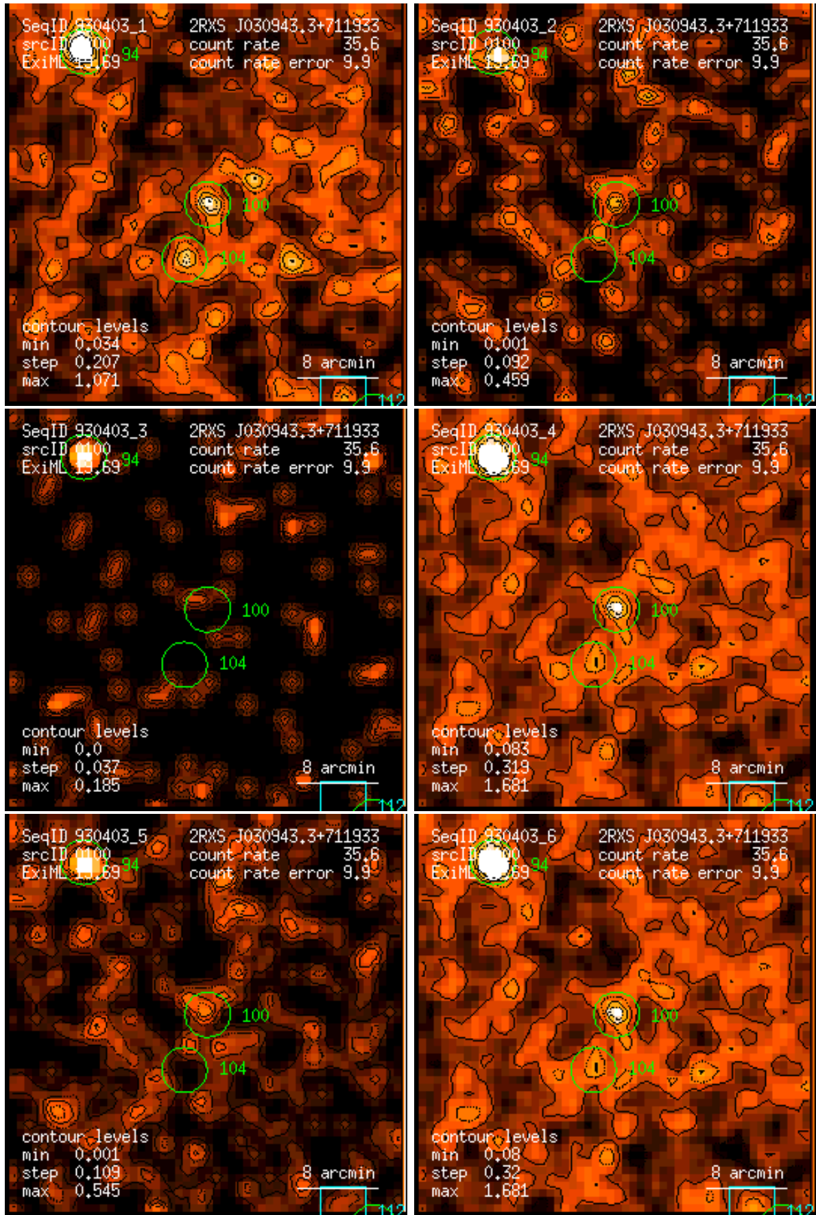
Figure 100: RASS 930403: detection 0100: band rate images, Gaussian filter: (1) PSPC channels 11 – 41, (2) 52 – 90, (3) 91 – 201, (4) 11 – 235, (5) 52 – 201, (6) 11 – 201. Broad band rates in counts/ks. Band rate contour levels in counts/ks/arcmin 2 .
