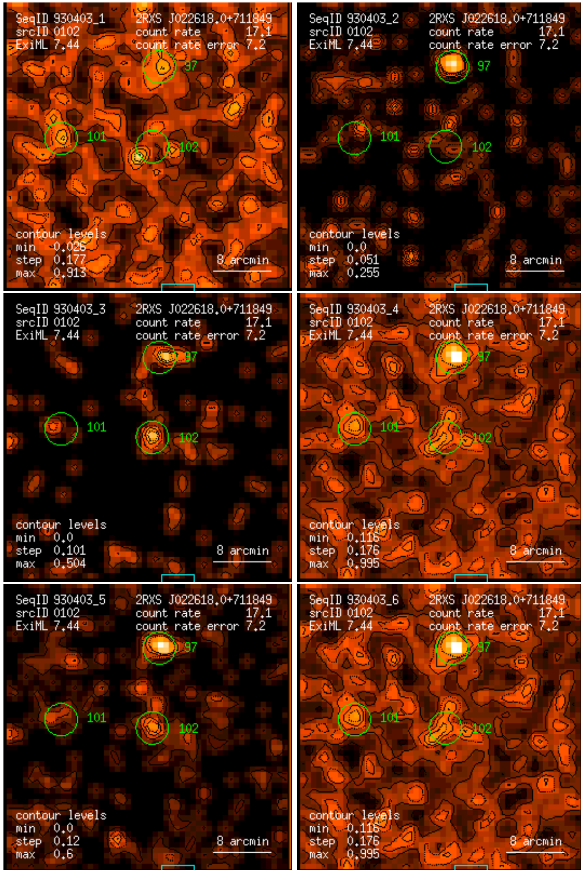
Figure 102: RASS 930403: detection 0102: band rate images, Gaussian filter: (1) PSPC channels 11 – 41, (2) 52 – 90, (3) 91 – 201, (4) 11 – 235, (5) 52 – 201, (6) 11 – 201. Broad band rates in counts/ks. Band rate contour levels in counts/ks/arcmin 2 .
