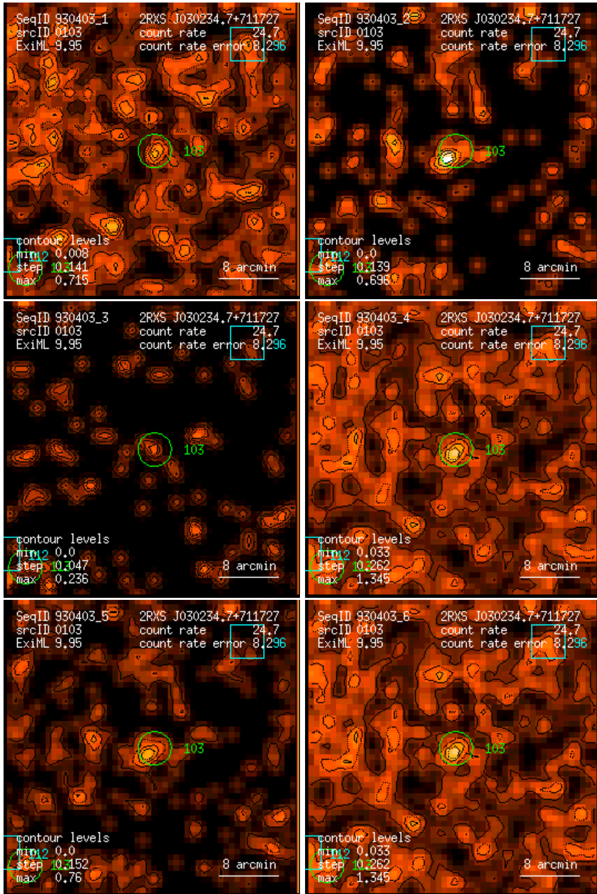
Figure 103: RASS 930403: detection 0103: band rate images, Gaussian filter: (1) PSPC channels 11 – 41, (2) 52 – 90, (3) 91 – 201, (4) 11 – 235, (5) 52 – 201, (6) 11 – 201. Broad band rates in counts/ks. Band rate contour levels in counts/ks/arcmin 2 .
