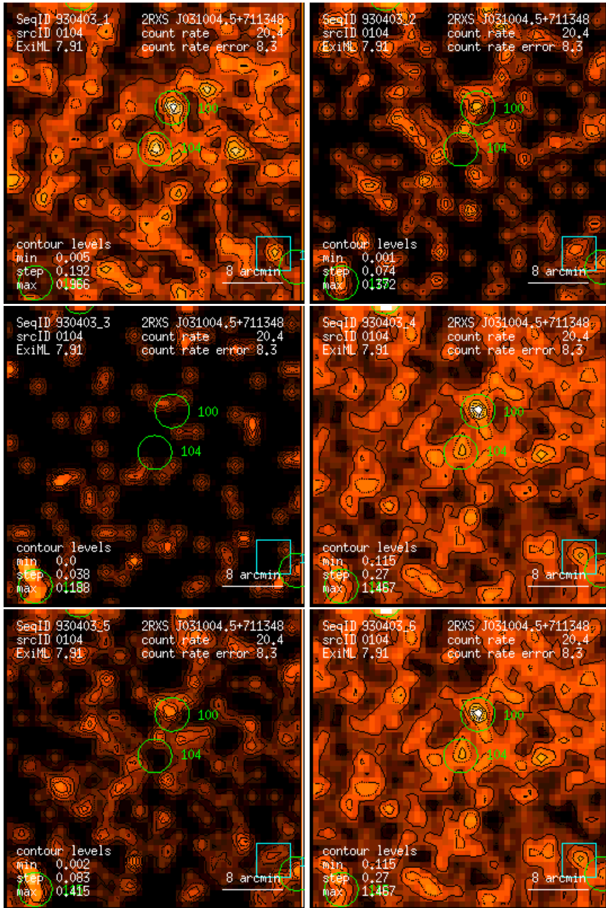
Figure 104: RASS 930403: detection 0104: band rate images, Gaussian filter: (1) PSPC channels 11 – 41, (2) 52 – 90, (3) 91 – 201, (4) 11 – 235, (5) 52 – 201, (6) 11 – 201. Broad band rates in counts/ks. Band rate contour levels in counts/ks/arcmin 2 .
