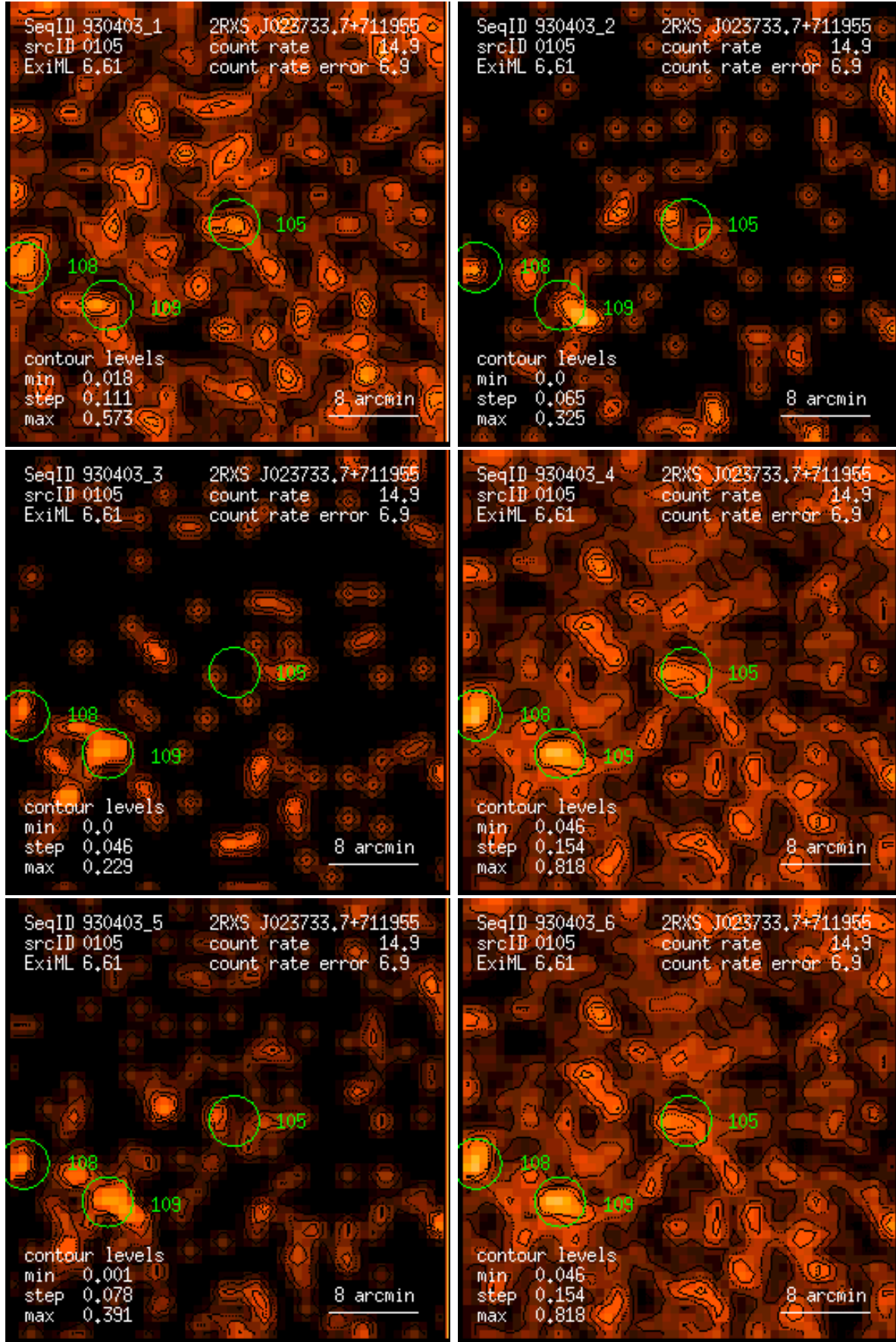
Figure 105: RASS 930403: detection 0105: band rate images, Gaussian filter: (1) PSPC channels 11 – 41, (2) 52 – 90, (3) 91 – 201, (4) 11 – 235, (5) 52 – 201, (6) 11 – 201. Broad band rates in counts/ks. Band rate contour levels in counts/ks/arcmin 2 .
