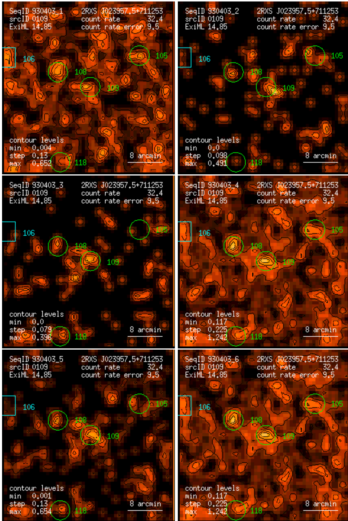
Figure 109: RASS 930403: detection 0109: band rate images, Gaussian filter: (1) PSPC channels 11 – 41, (2) 52 – 90, (3) 91 – 201, (4) 11 – 235, (5) 52 – 201, (6) 11 – 201. Broad band rates in counts/ks. Band rate contour levels in counts/ks/arcmin 2 .
