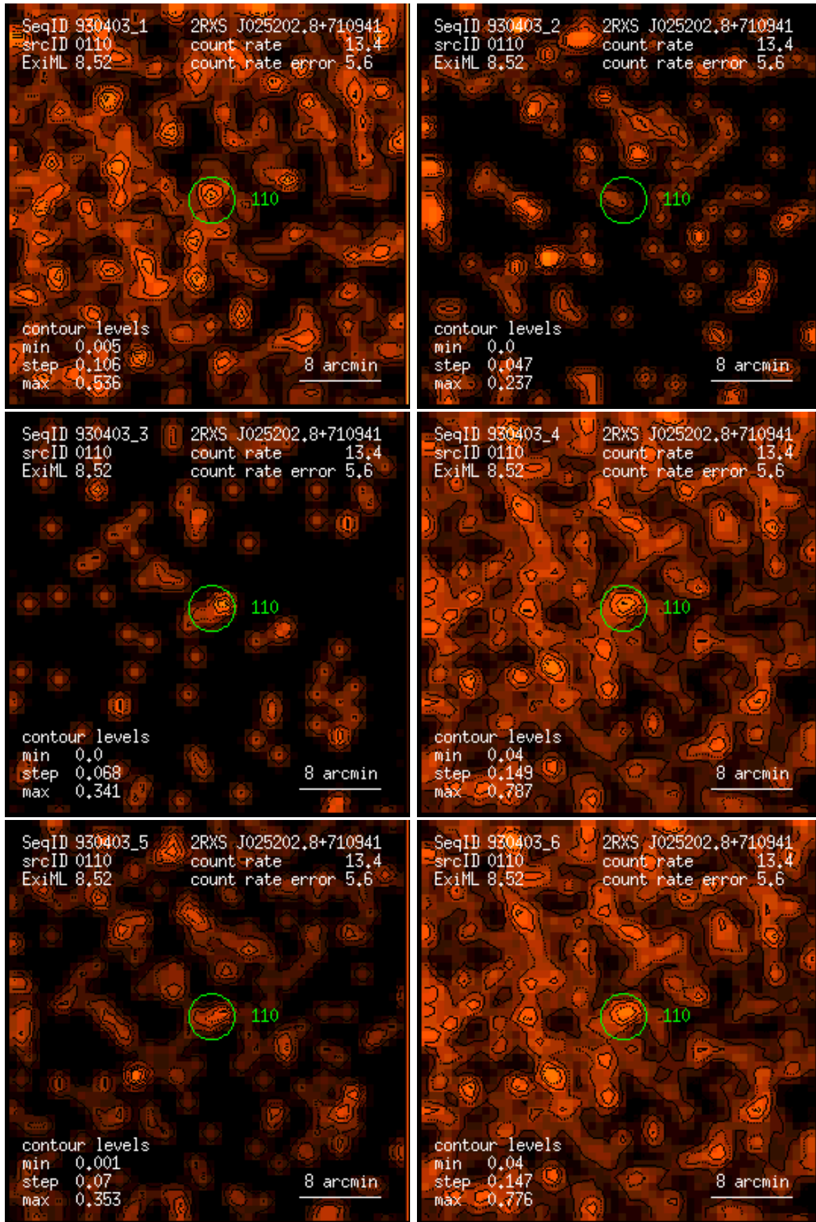
Figure 110: RASS 930403: detection 0110: band rate images, Gaussian filter: (1) PSPC channels 11 – 41, (2) 52 – 90, (3) 91 – 201, (4) 11 – 235, (5) 52 – 201, (6) 11 – 201. Broad band rates in counts/ks. Band rate contour levels in counts/ks/arcmin 2 .
