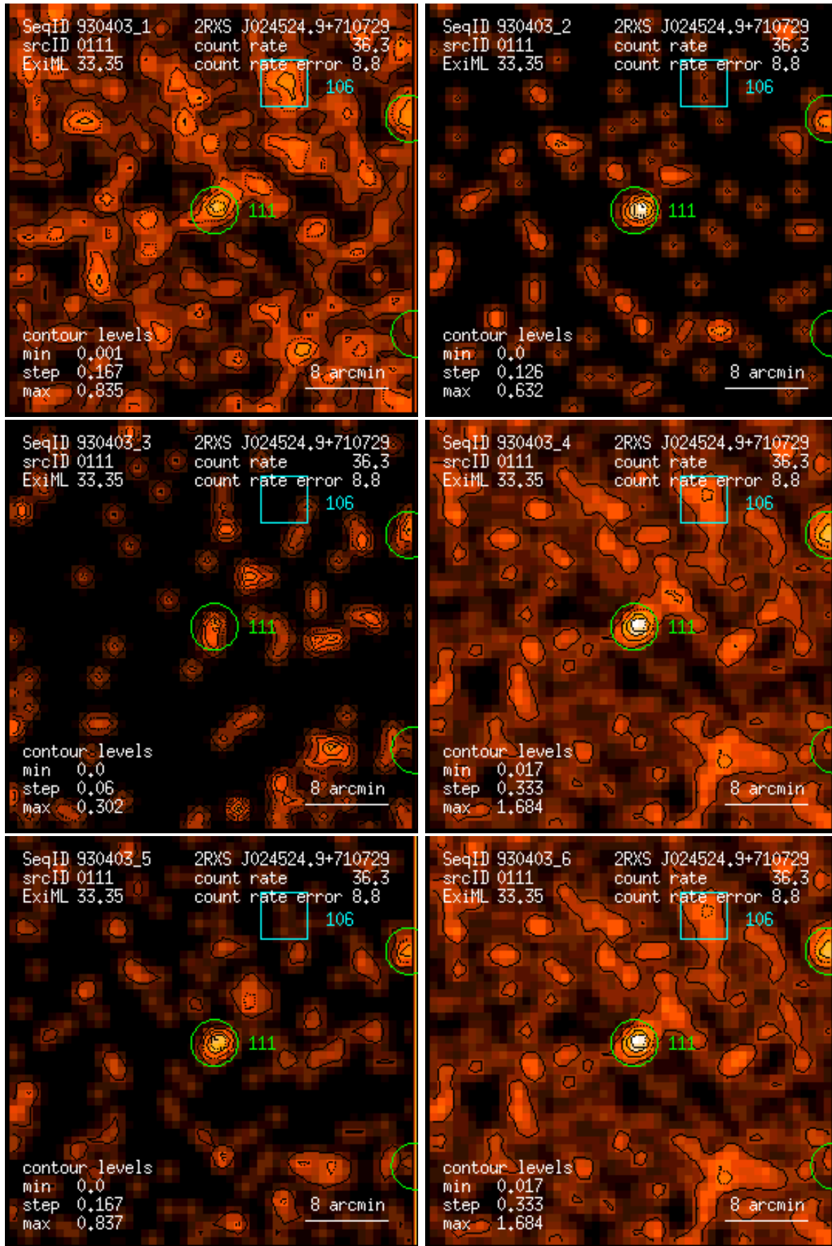
Figure 111: RASS 930403: detection 0111: band rate images, Gaussian filter: (1) PSPC channels 11 – 41, (2) 52 – 90, (3) 91 – 201, (4) 11 – 235, (5) 52 – 201, (6) 11 – 201. Broad band rates in counts/ks. Band rate contour levels in counts/ks/arcmin 2 .
