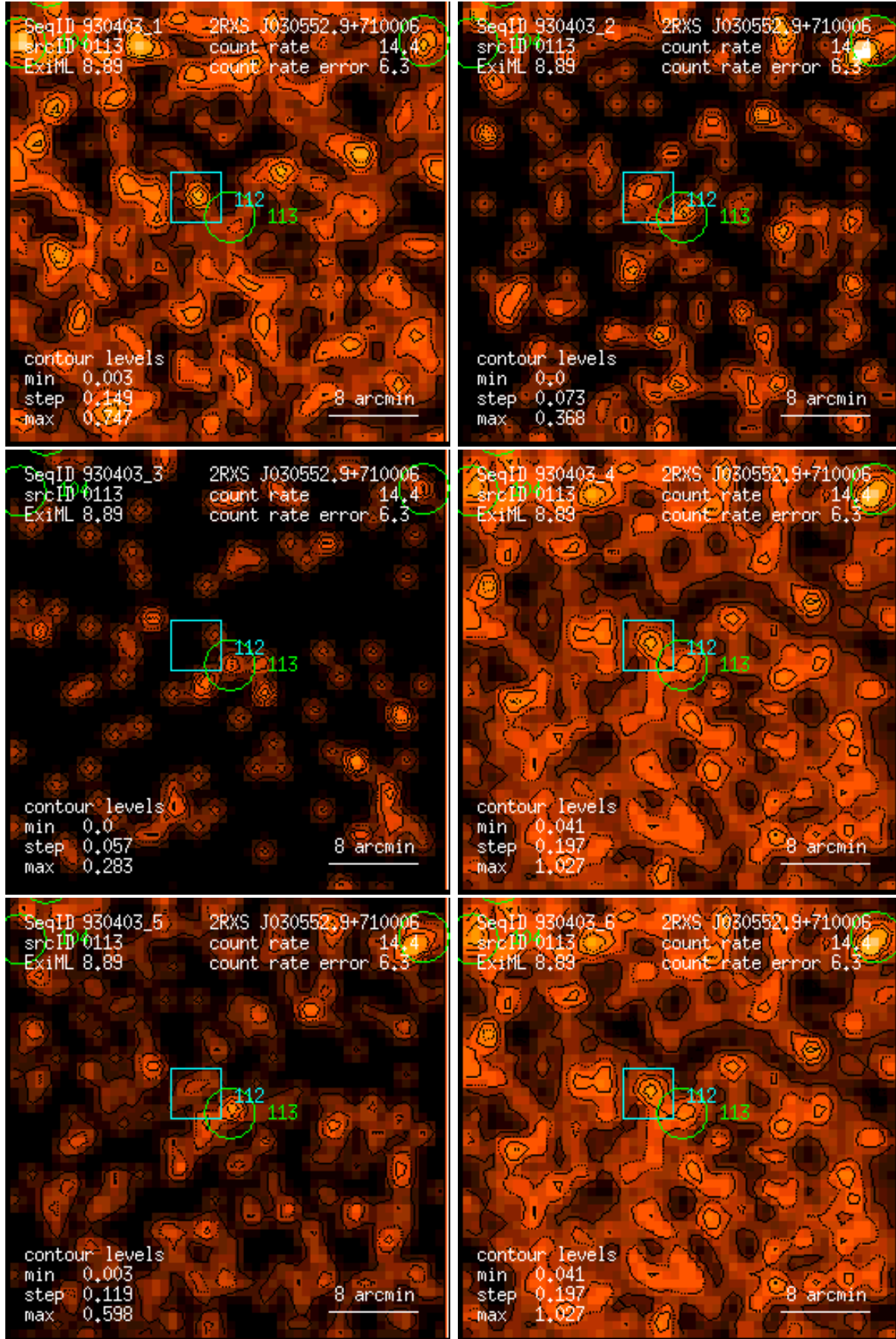
Figure 113: RASS 930403: detection 0113: band rate images, Gaussian filter: (1) PSPC channels 11 – 41, (2) 52 – 90, (3) 91 – 201, (4) 11 – 235, (5) 52 – 201, (6) 11 – 201. Broad band rates in counts/ks. Band rate contour levels in counts/ks/arcmin 2 .
