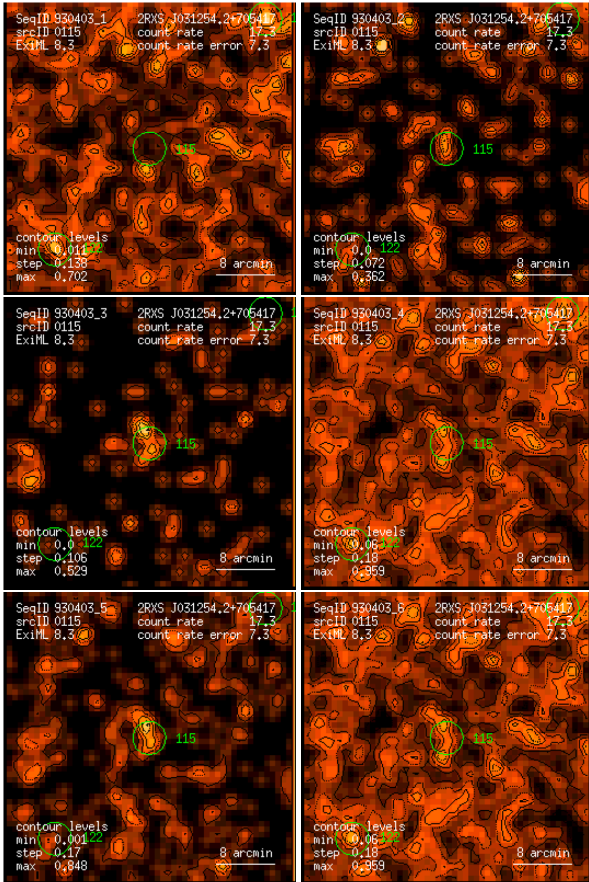
Figure 115: RASS 930403: detection 0115: band rate images, Gaussian filter: (1) PSPC channels 11 – 41, (2) 52 – 90, (3) 91 – 201, (4) 11 – 235, (5) 52 – 201, (6) 11 – 201. Broad band rates in counts/ks. Band rate contour levels in counts/ks/arcmin 2 .
