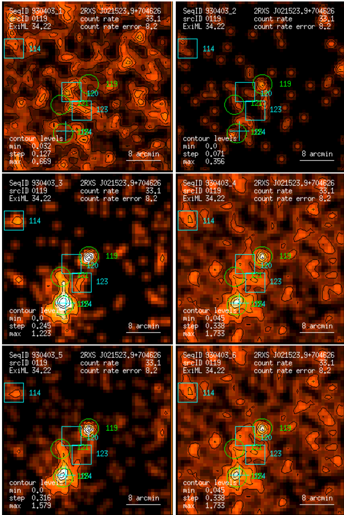
Figure 119: RASS 930403: detection 0119: band rate images, Gaussian filter: (1) PSPC channels 11 – 41, (2) 52 – 90, (3) 91 – 201, (4) 11 – 235, (5) 52 – 201, (6) 11 – 201. Broad band rates in counts/ks. Band rate contour levels in counts/ks/arcmin 2 .
