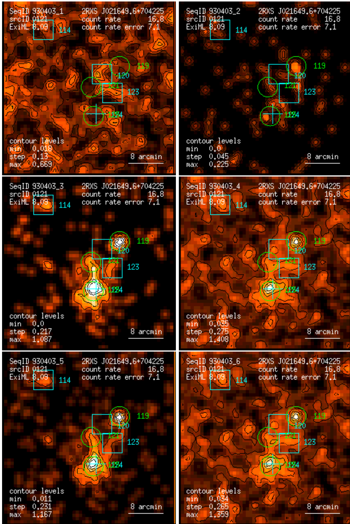
Figure 121: RASS 930403: detection 0121: band rate images, Gaussian filter: (1) PSPC channels 11 – 41, (2) 52 – 90, (3) 91 – 201, (4) 11 – 235, (5) 52 – 201, (6) 11 – 201. Broad band rates in counts/ks. Band rate contour levels in counts/ks/arcmin 2 .
