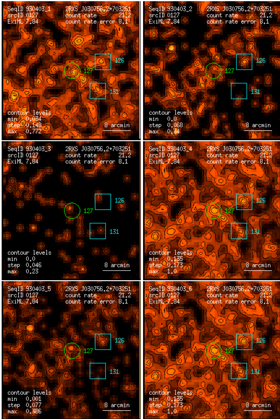
Figure 127: RASS 930403: detection 0127: band rate images, Gaussian filter: (1) PSPC channels 11 – 41, (2) 52 – 90, (3) 91 – 201, (4) 11 – 235, (5) 52 – 201, (6) 11 – 201. Broad band rates in counts/ks. Band rate contour levels in counts/ks/arcmin 2 .
