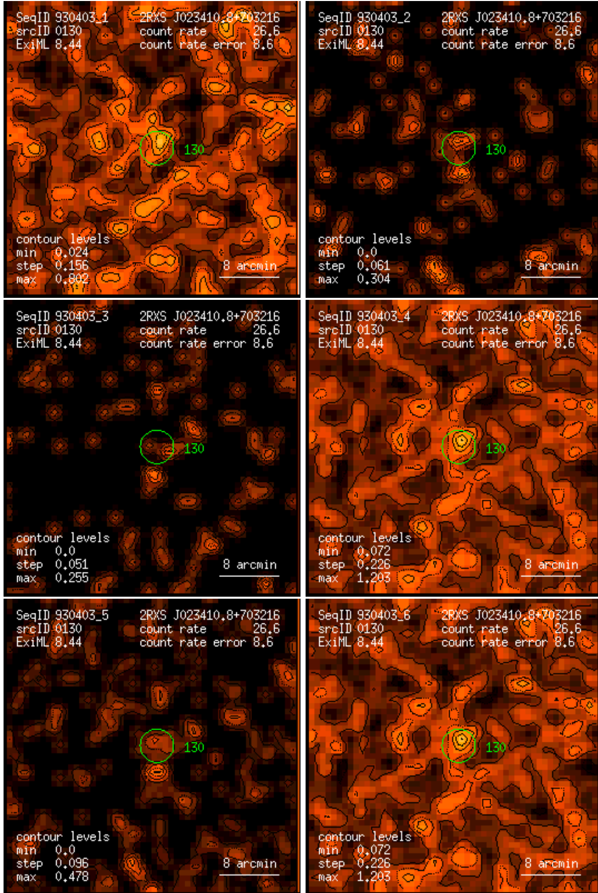
Figure 130: RASS 930403: detection 0130: band rate images, Gaussian filter: (1) PSPC channels 11 – 41, (2) 52 – 90, (3) 91 – 201, (4) 11 – 235, (5) 52 – 201, (6) 11 – 201. Broad band rates in counts/ks. Band rate contour levels in counts/ks/arcmin 2 .
