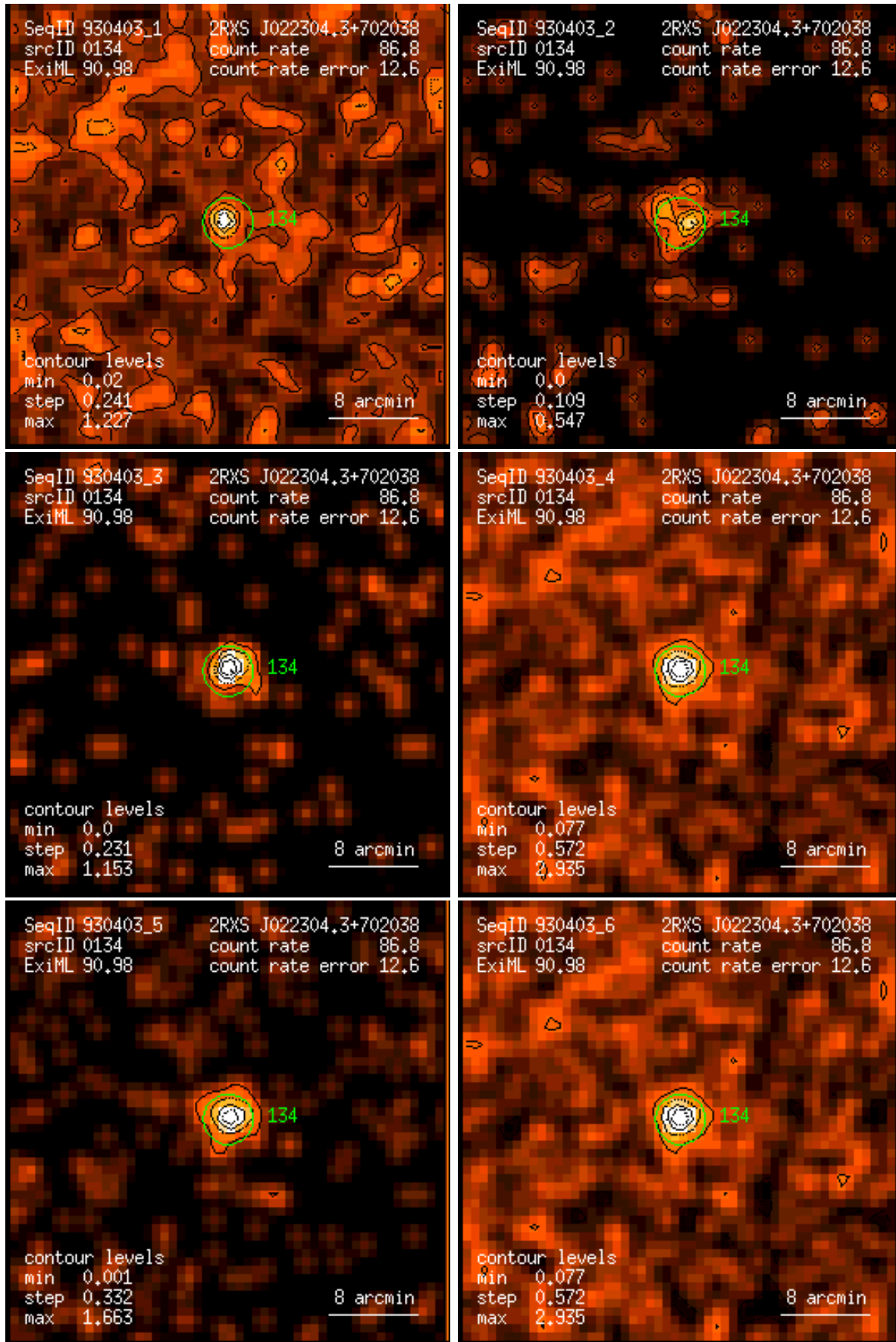
Figure 134: RASS 930403: detection 0134: band rate images, Gaussian filter: (1) PSPC channels 11 – 41, (2) 52 – 90, (3) 91 – 201, (4) 11 – 235, (5) 52 – 201, (6) 11 – 201. Broad band rates in counts/ks. Band rate contour levels in counts/ks/arcmin 2 .
