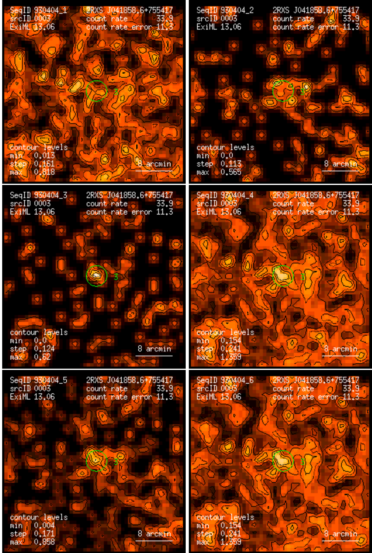
Figure 3: RASS 930404: detection 0003: band rate images, Gaussian filter: (1) PSPC channels 11 – 41, (2) 52 – 90, (3) 91 – 201, (4) 11 – 235, (5) 52 – 201, (6) 11 – 201. Broad band rates in counts/ks. Band rate contour levels in counts/ks/arcmin 2 .
