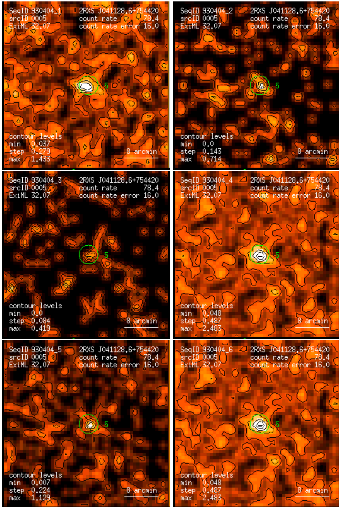
Figure 5: RASS 930404: detection 0005: band rate images, Gaussian filter: (1) PSPC channels 11 – 41, (2) 52 – 90, (3) 91 – 201, (4) 11 – 235, (5) 52 – 201, (6) 11 – 201. Broad band rates in counts/ks. Band rate contour levels in counts/ks/arcmin 2 .
