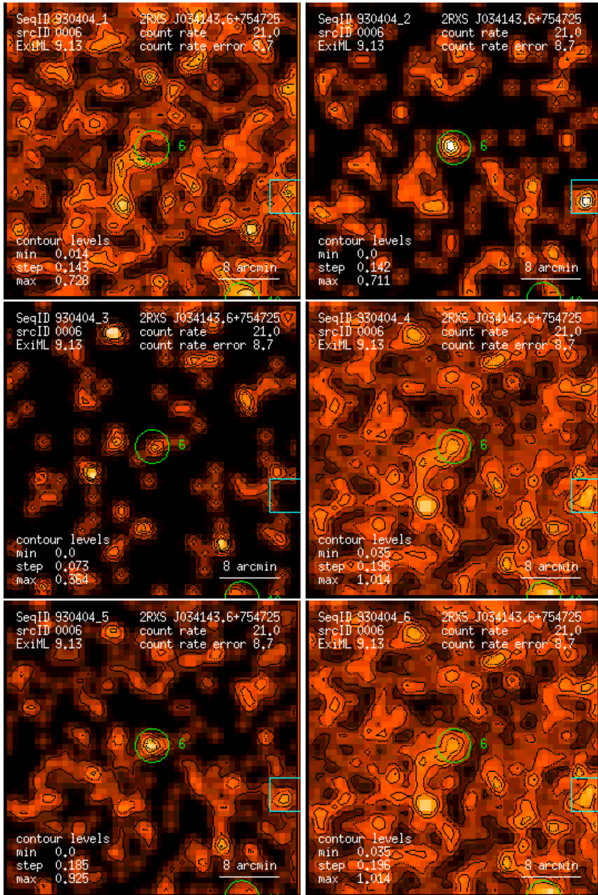
Figure 6: RASS 930404: detection 0006: band rate images, Gaussian filter: (1) PSPC channels 11 – 41, (2) 52 – 90, (3) 91 – 201, (4) 11 – 235, (5) 52 – 201, (6) 11 – 201. Broad band rates in counts/ks. Band rate contour levels in counts/ks/arcmin 2 .
