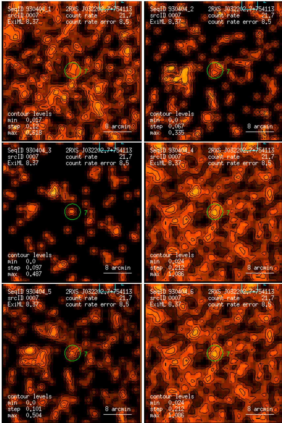
Figure 7: RASS 930404: detection 0007: band rate images, Gaussian filter: (1) PSPC channels 11 – 41, (2) 52 – 90, (3) 91 – 201, (4) 11 – 235, (5) 52 – 201, (6) 11 – 201. Broad band rates in counts/ks. Band rate contour levels in counts/ks/arcmin 2 .
