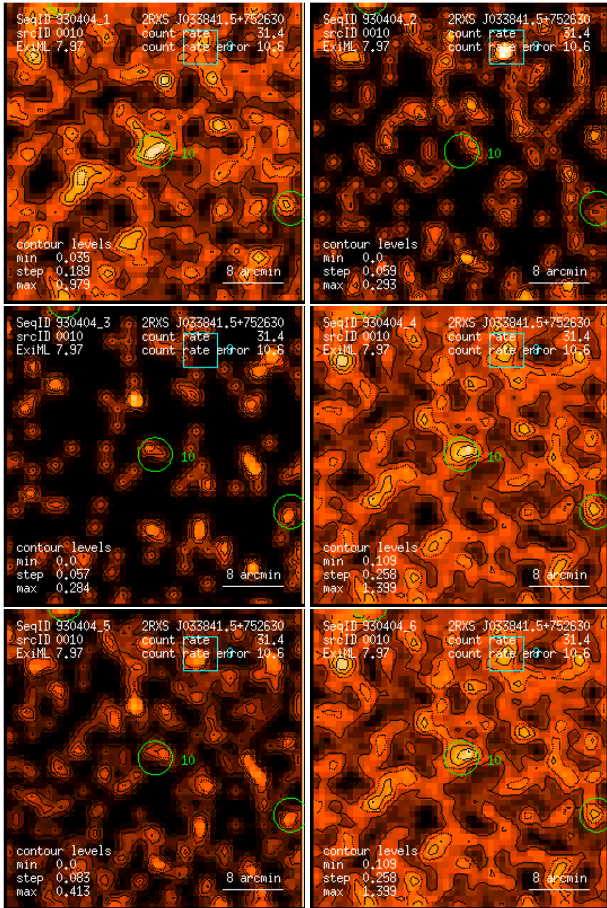
Figure 10: RASS 930404: detection 0010: band rate images, Gaussian filter: (1) PSPC channels 11 – 41, (2) 52 – 90, (3) 91 – 201, (4) 11 – 235, (5) 52 – 201, (6) 11 – 201. Broad band rates in counts/ks. Band rate contour levels in counts/ks/arcmin 2 .
