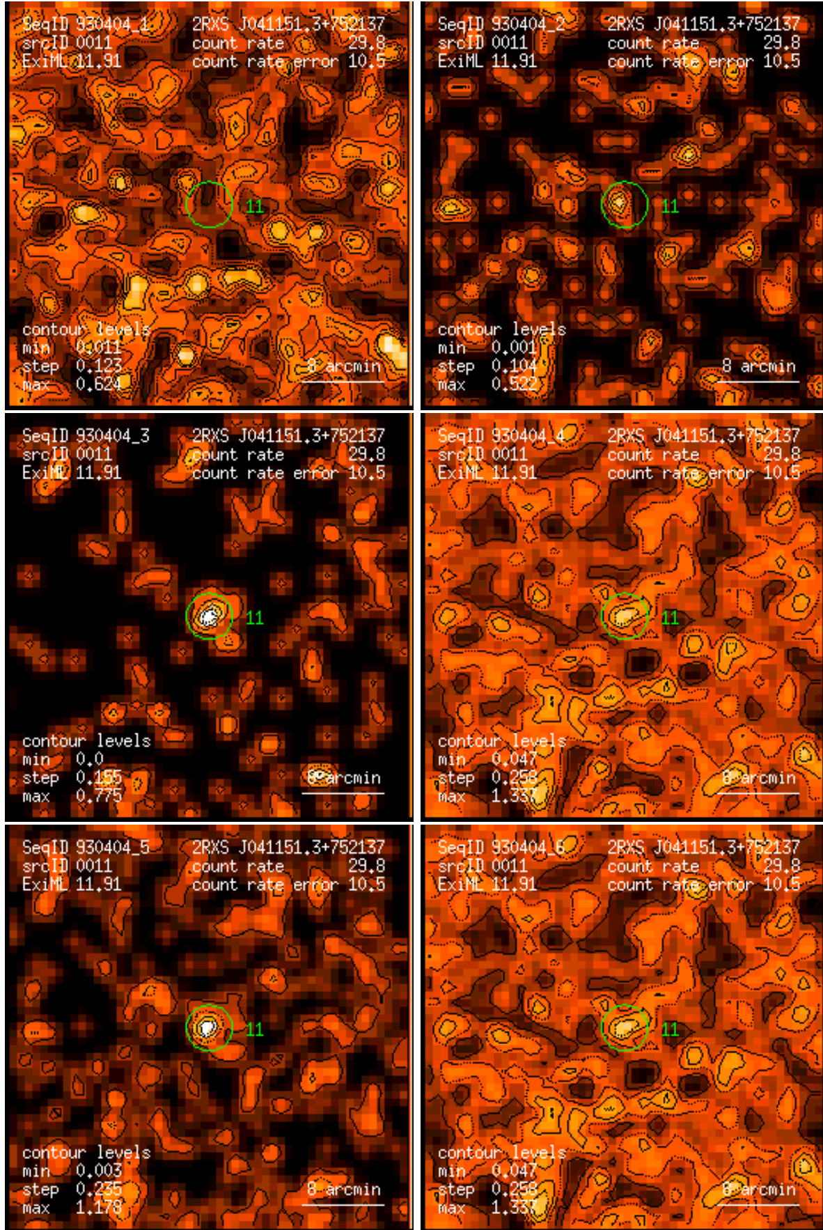
Figure 11: RASS 930404: detection 0011: band rate images, Gaussian filter: (1) PSPC channels 11 – 41, (2) 52 – 90, (3) 91 – 201, (4) 11 – 235, (5) 52 – 201, (6) 11 – 201. Broad band rates in counts/ks. Band rate contour levels in counts/ks/arcmin 2 .
