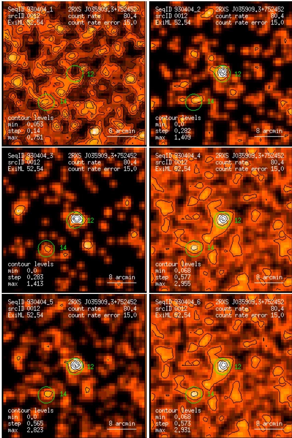
Figure 12: RASS 930404: detection 0012: band rate images, Gaussian filter: (1) PSPC channels 11 – 41, (2) 52 – 90, (3) 91 – 201, (4) 11 – 235, (5) 52 – 201, (6) 11 – 201. Broad band rates in counts/ks. Band rate contour levels in counts/ks/arcmin 2 .
