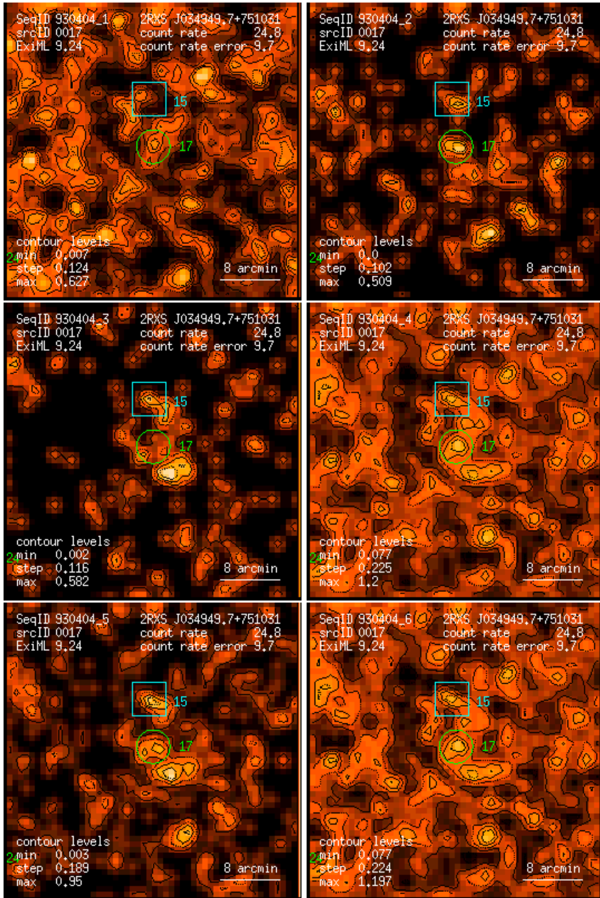
Figure 17: RASS 930404: detection 0017: band rate images, Gaussian filter: (1) PSPC channels 11 – 41, (2) 52 – 90, (3) 91 – 201, (4) 11 – 235, (5) 52 – 201, (6) 11 – 201. Broad band rates in counts/ks. Band rate contour levels in counts/ks/arcmin 2 .
