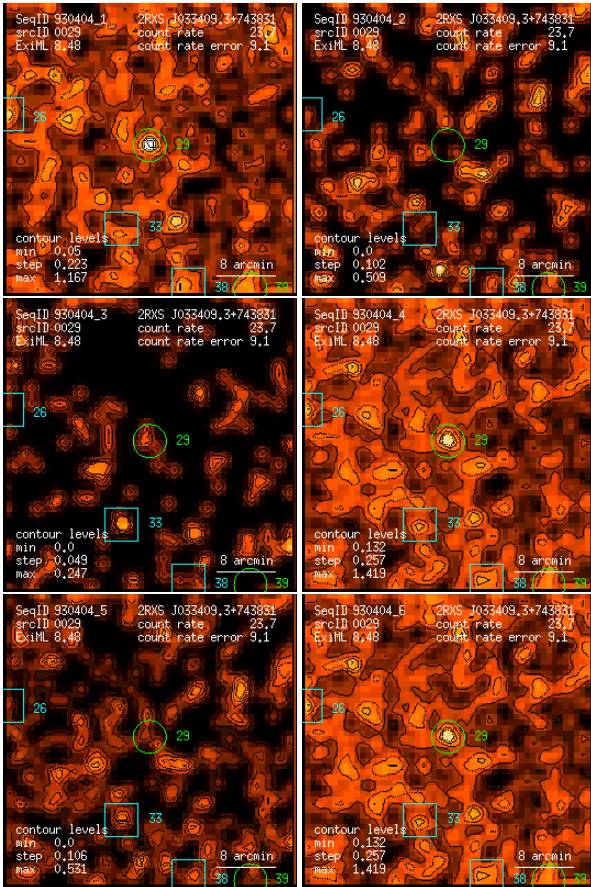
Figure 29: RASS 930404: detection 0029: band rate images, Gaussian filter: (1) PSPC channels 11 – 41, (2) 52 – 90, (3) 91 – 201, (4) 11 – 235, (5) 52 – 201, (6) 11 – 201. Broad band rates in counts/ks. Band rate contour levels in counts/ks/arcmin 2 .
