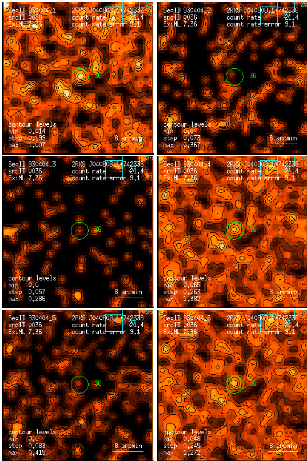
Figure 36: RASS 930404: detection 0036: band rate images, Gaussian filter: (1) PSPC channels 11 – 41, (2) 52 – 90, (3) 91 – 201, (4) 11 – 235, (5) 52 – 201, (6) 11 – 201. Broad band rates in counts/ks. Band rate contour levels in counts/ks/arcmin 2 .
