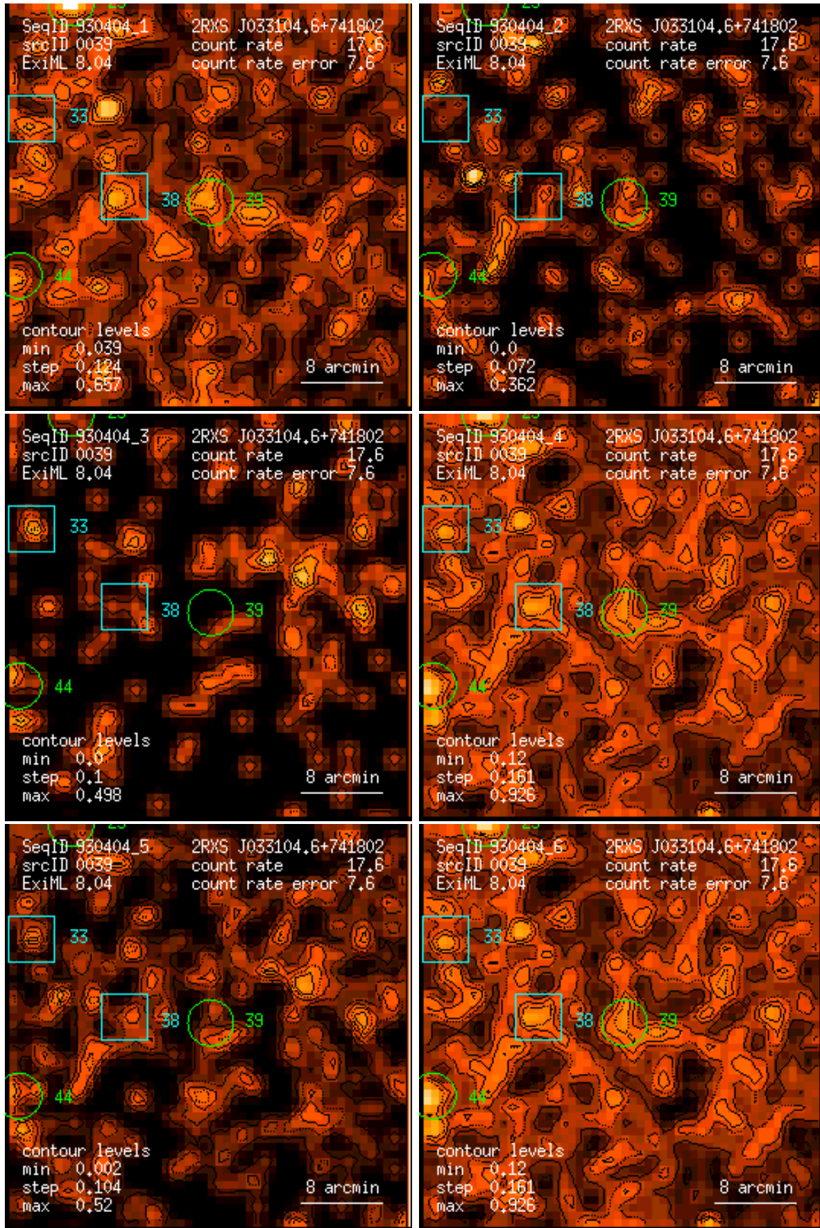
Figure 39: RASS 930404: detection 0039: band rate images, Gaussian filter: (1) PSPC channels 11 – 41, (2) 52 – 90, (3) 91 – 201, (4) 11 – 235, (5) 52 – 201, (6) 11 – 201. Broad band rates in counts/ks. Band rate contour levels in counts/ks/arcmin 2 .
