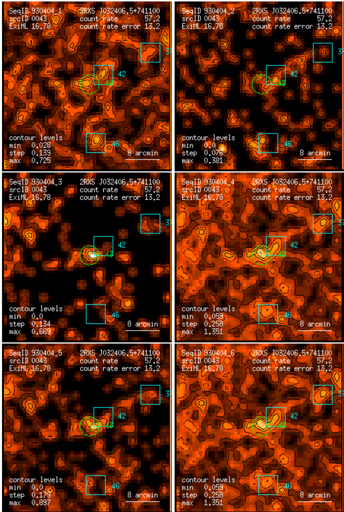
Figure 43: RASS 930404: detection 0043: band rate images, Gaussian filter: (1) PSPC channels 11 – 41, (2) 52 – 90, (3) 91 – 201, (4) 11 – 235, (5) 52 – 201, (6) 11 – 201. Broad band rates in counts/ks. Band rate contour levels in counts/ks/arcmin 2 .
