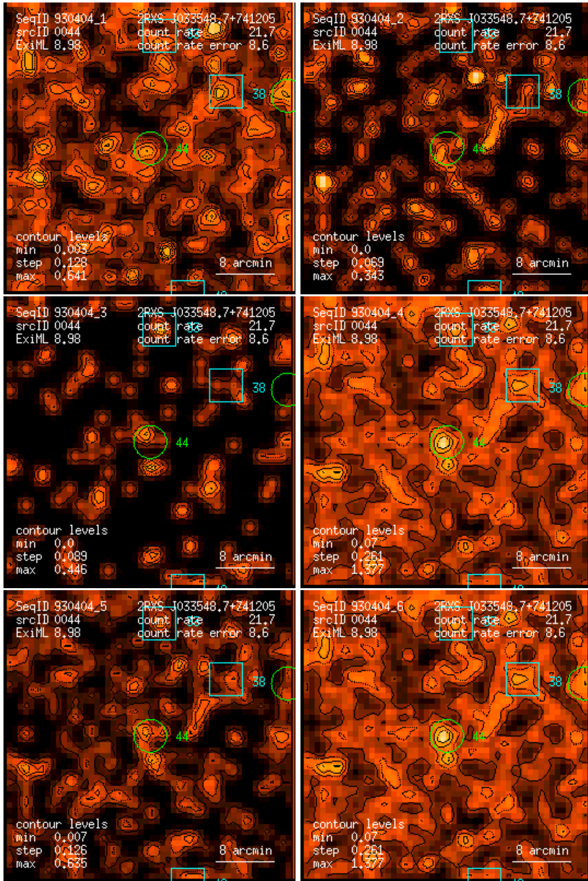
Figure 44: RASS 930404: detection 0044: band rate images, Gaussian filter: (1) PSPC channels 11 – 41, (2) 52 – 90, (3) 91 – 201, (4) 11 – 235, (5) 52 – 201, (6) 11 – 201. Broad band rates in counts/ks. Band rate contour levels in counts/ks/arcmin 2 .
