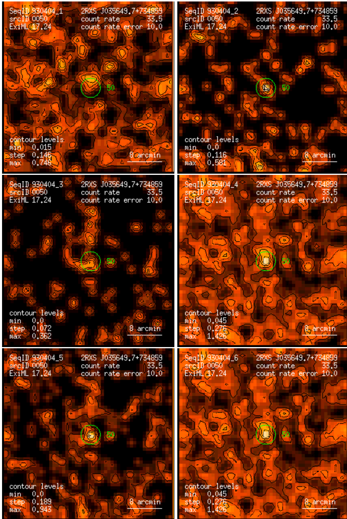
Figure 50: RASS 930404: detection 0050: band rate images, Gaussian filter: (1) PSPC channels 11 – 41, (2) 52 – 90, (3) 91 – 201, (4) 11 – 235, (5) 52 – 201, (6) 11 – 201. Broad band rates in counts/ks. Band rate contour levels in counts/ks/arcmin 2 .
