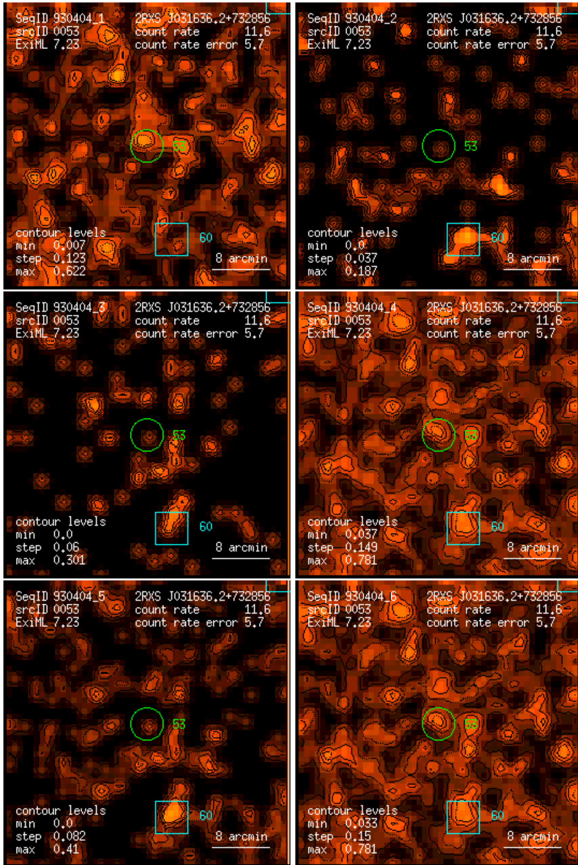
Figure 53: RASS 930404: detection 0053: band rate images, Gaussian filter: (1) PSPC channels 11 – 41, (2) 52 – 90, (3) 91 – 201, (4) 11 – 235, (5) 52 – 201, (6) 11 – 201. Broad band rates in counts/ks. Band rate contour levels in counts/ks/arcmin 2 .
