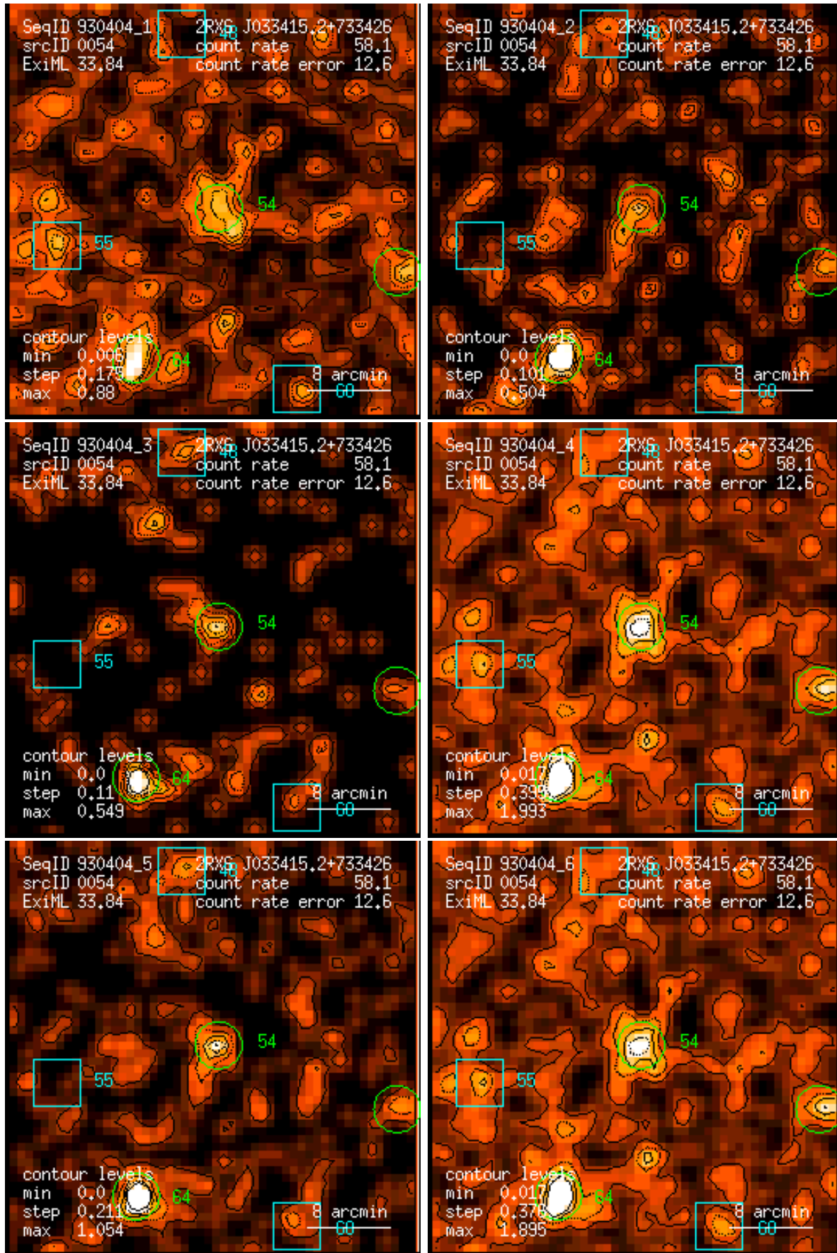
Figure 54: RASS 930404: detection 0054: band rate images, Gaussian filter: (1) PSPC channels 11 – 41, (2) 52 – 90, (3) 91 – 201, (4) 11 – 235, (5) 52 – 201, (6) 11 – 201. Broad band rates in counts/ks. Band rate contour levels in counts/ks/arcmin 2 .
