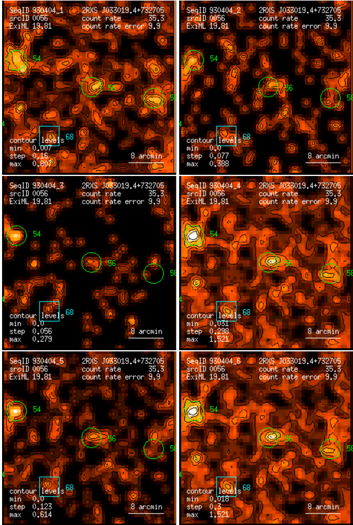
Figure 56: RASS 930404: detection 0056: band rate images, Gaussian filter: (1) PSPC channels 11 – 41, (2) 52 – 90, (3) 91 – 201, (4) 11 – 235, (5) 52 – 201, (6) 11 – 201. Broad band rates in counts/ks. Band rate contour levels in counts/ks/arcmin 2 .
