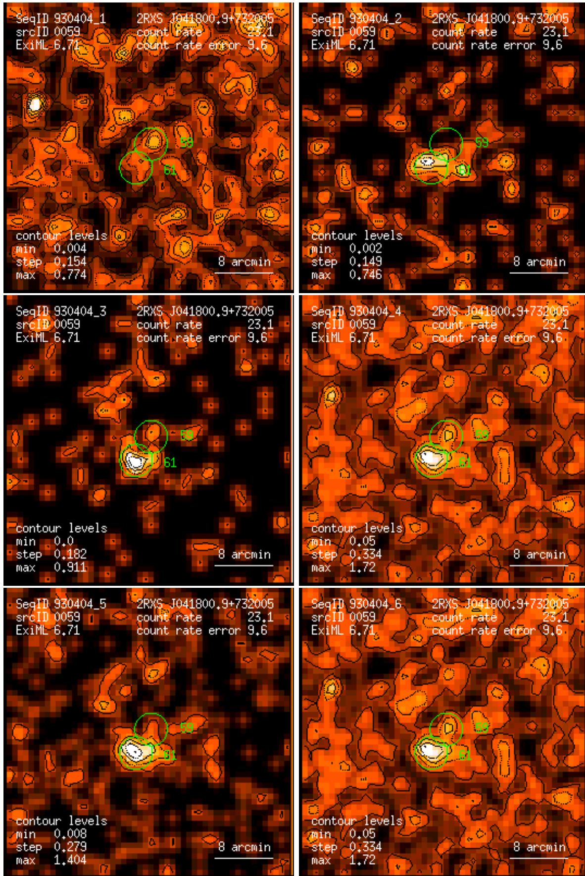
Figure 59: RASS 930404: detection 0059: band rate images, Gaussian filter: (1) PSPC channels 11 – 41, (2) 52 – 90, (3) 91 – 201, (4) 11 – 235, (5) 52 – 201, (6) 11 – 201. Broad band rates in counts/ks. Band rate contour levels in counts/ks/arcmin 2 .
